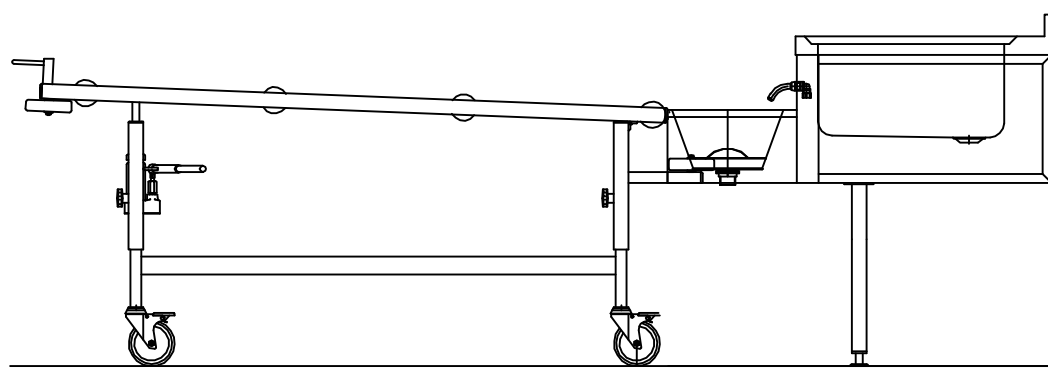
SECTION THROUGH BOWL UNIT
